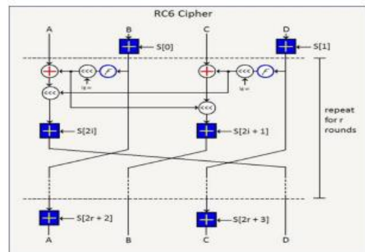
Fig 4: General Diagram of RC6 Algorithm
