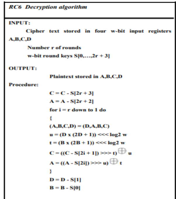
Fig 7: Decryption algorithm of RC6
