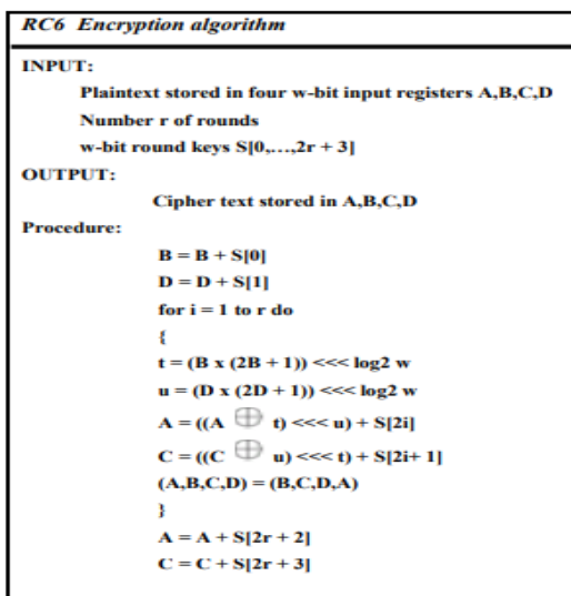
Fig 6: Encryption algorithm of RC6
