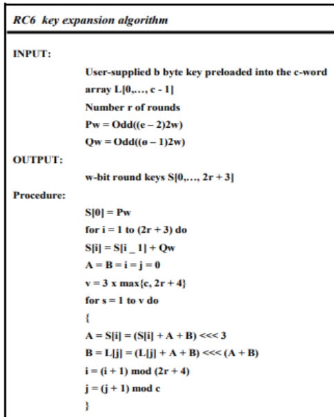
Fig 5: Key Expansion Algorithm of RC6
